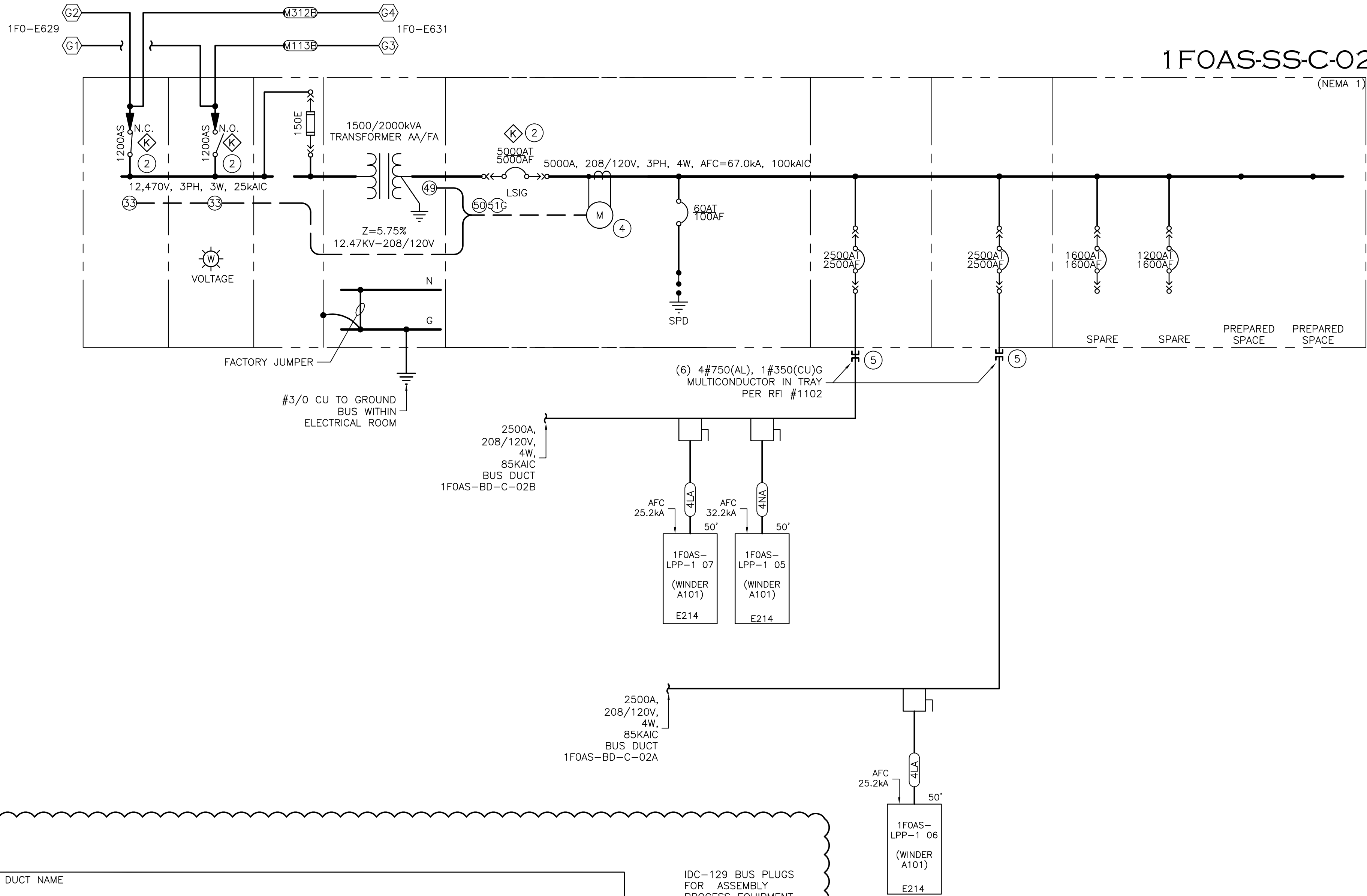
1 ONE LINE DIAGRAM - (1FO) ASSEMBLY-2 "C" (PARTIAL) NO SCALE
